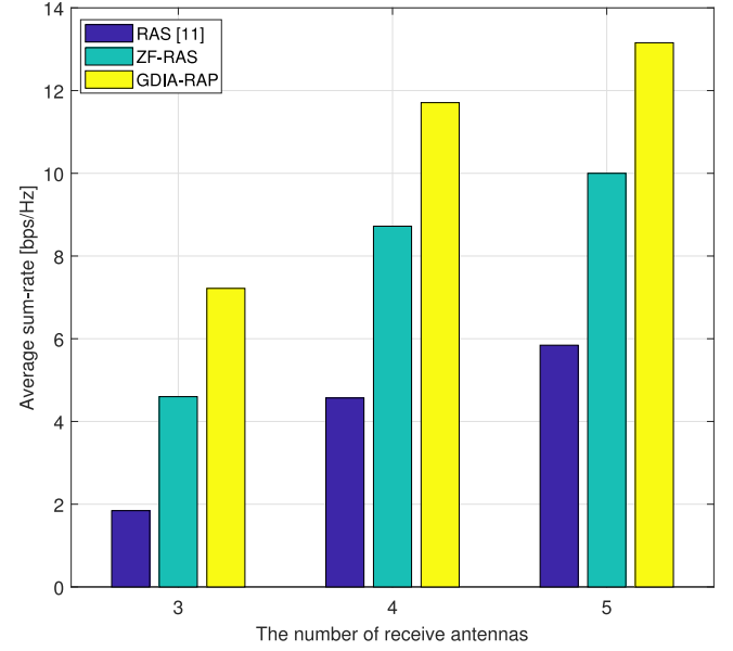
Fig. 1. Average sum-rate comparison when K = 2 , M = 3 , L_{ID} = 2 , S = 2 , SNR = 10 dB, and Q_{req} = 0.3 .
